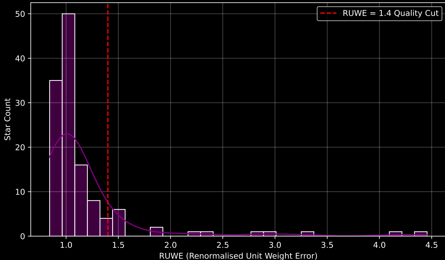
GALAH DR4 Field [3971] RUWE Distribution (n= 128)
