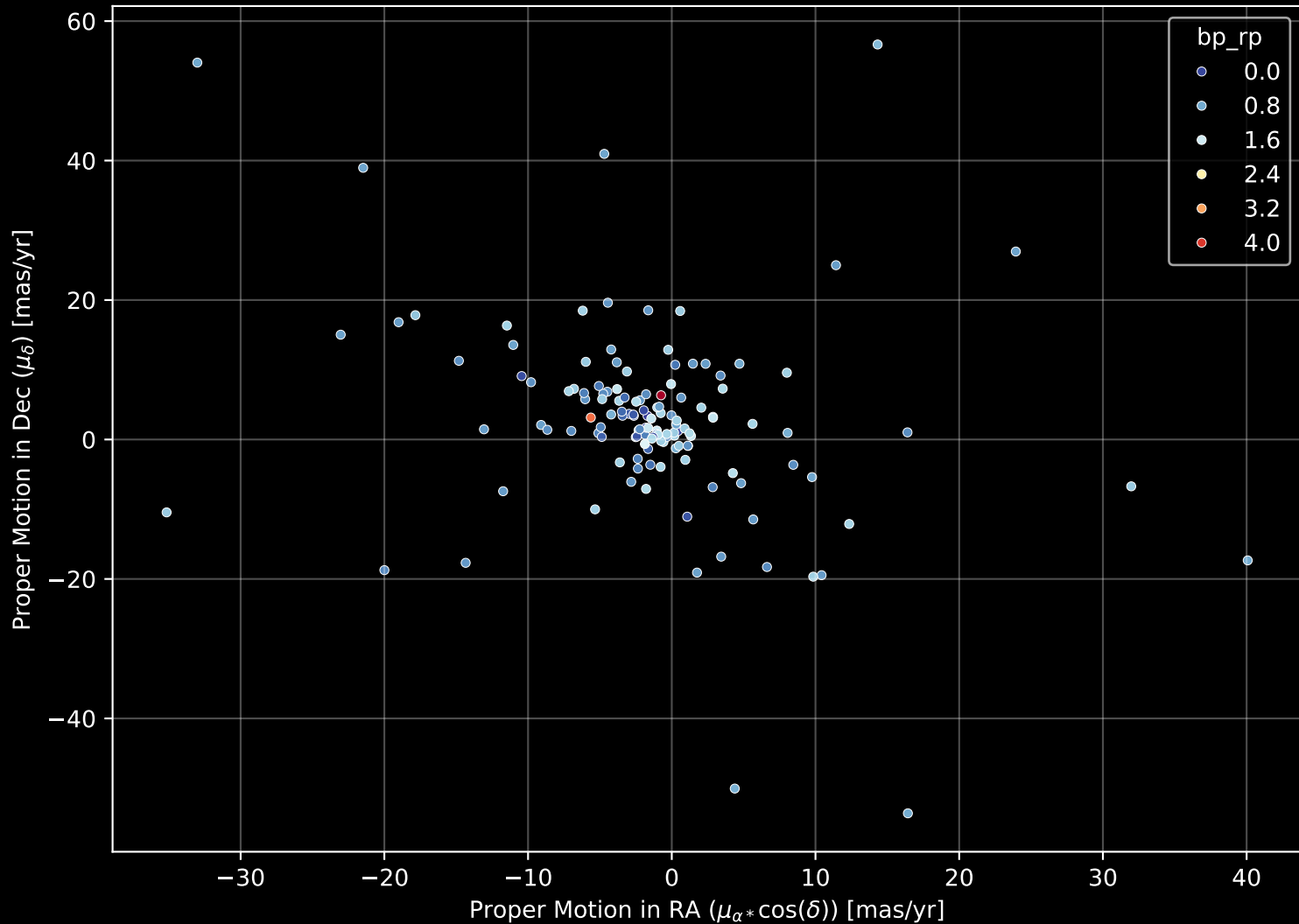
GALAH DR4 Field: [3971] Proper Motion Diagram (n= 134)
