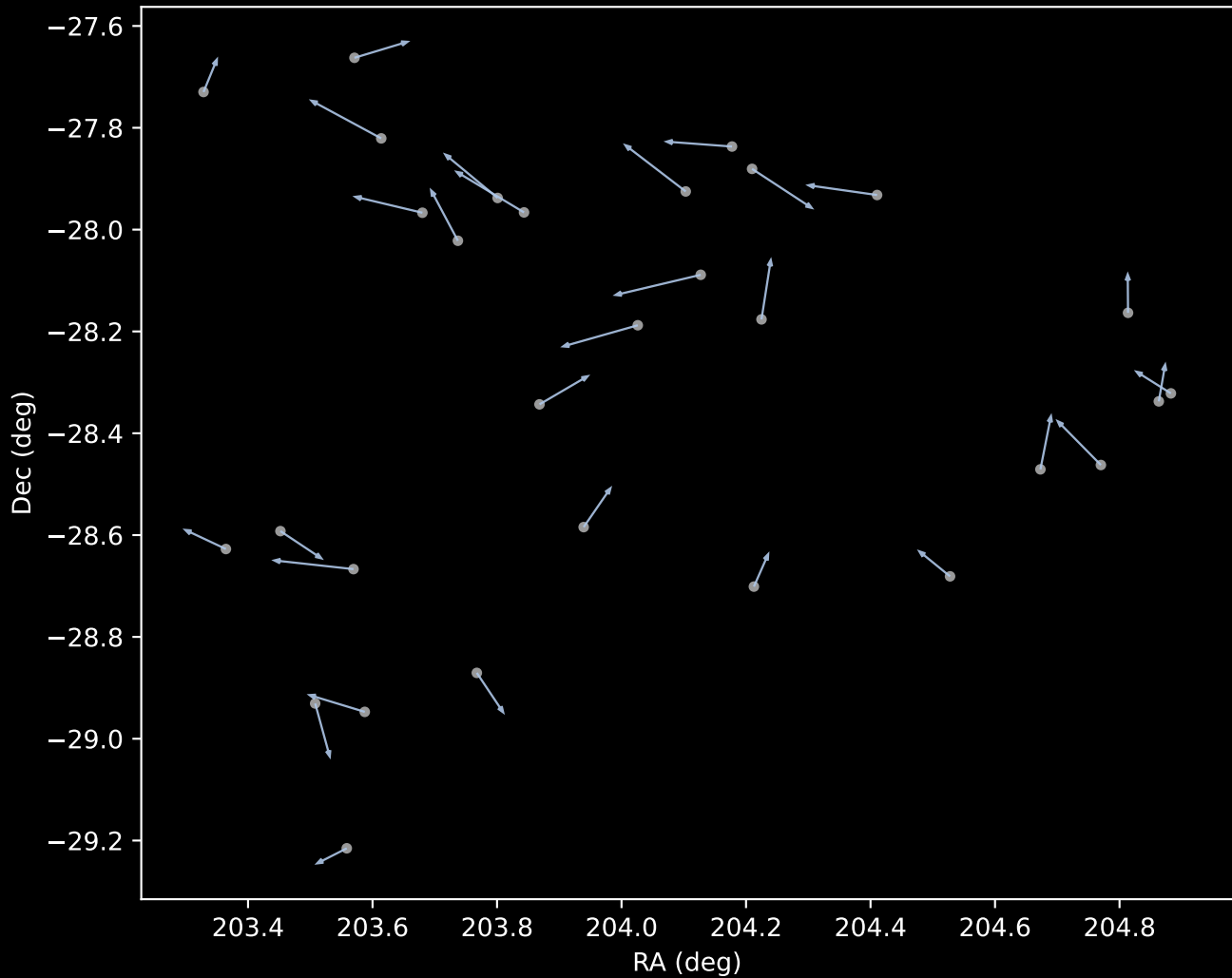
GALAH DR4 Cluster 1 Proper Motion Vectors (n=30)
