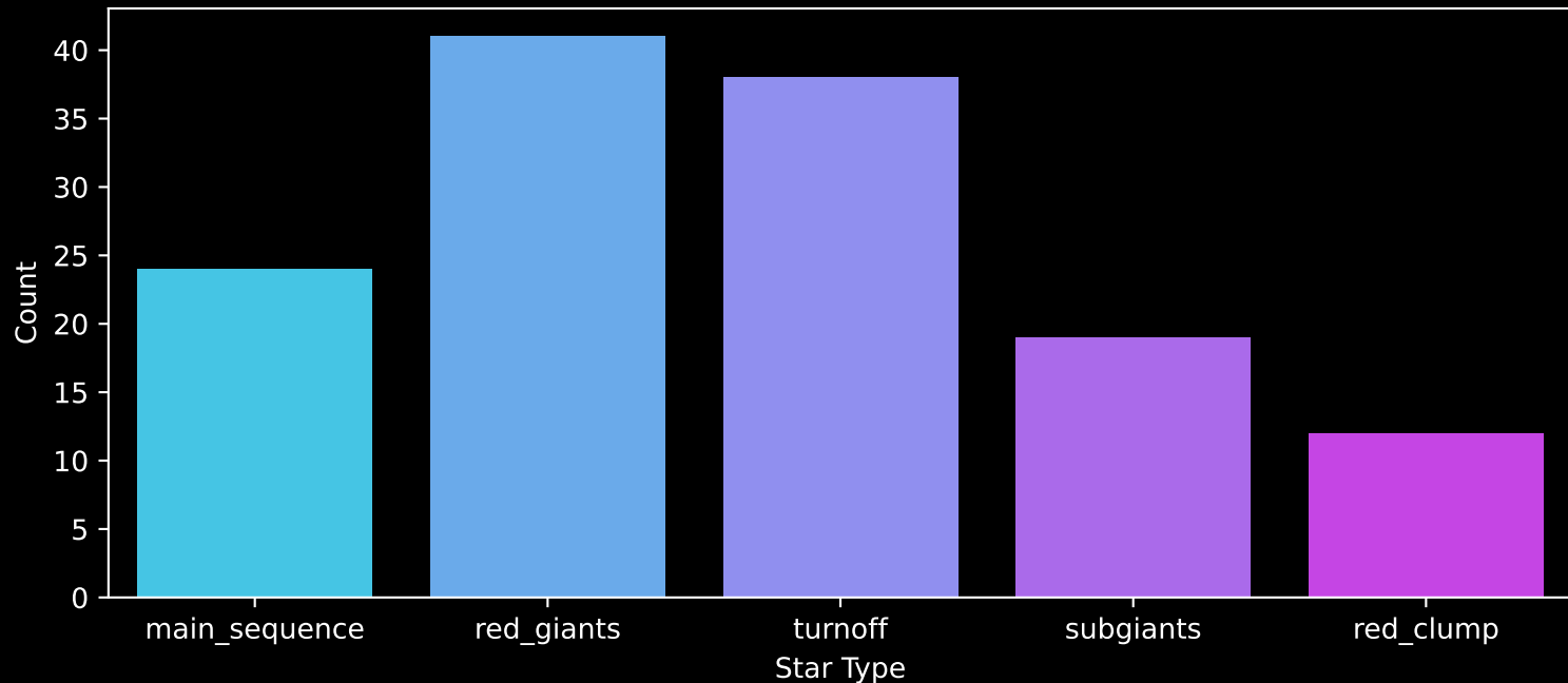
GALAH DR4 Field: [3971] Count plot of Star Type
